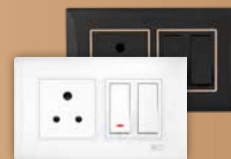
MARVEL
